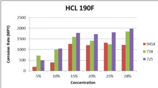
Figure 12: Weight loss of alloys 945X®, 718 and 725 at various HCl concentrations at 190°F [88°C]
