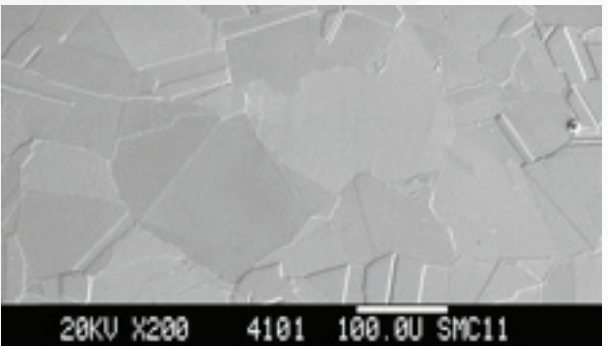
Figure 17: Scanning electron micrographs of 10-inch [254 mm] diameter alloy 945X® rod at center in longitudinal orientation.
