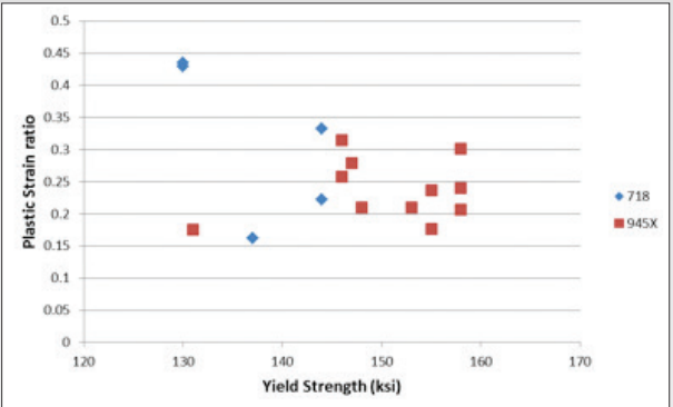
Figure 10 shows plastic strain ratios of alloy 945X ® and 718 in glycerol and in the listed hydrogen embrittlement environment. The latter is divided by the former to get these values.
