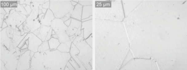
Figure 16: Optical photographs of 22-inch [560 mm] diameter rod of alloy 945X® at center in longitudinal orientation.
