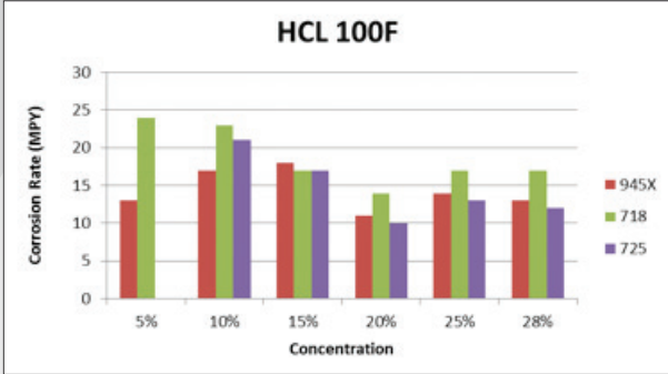
Figure 11: Weight loss of alloys 945X®, 718 and 725 at various HCl concentrations 100°F [38°C]
