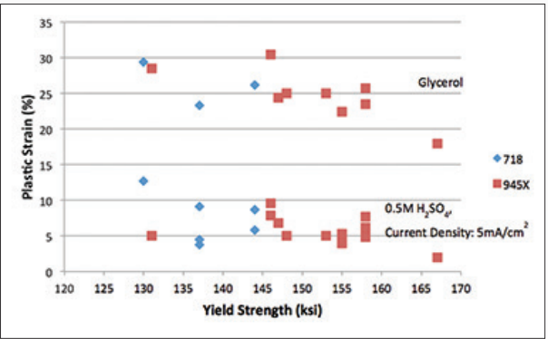
Figure 9 shows plastic strains of alloy 945X ® and 718 in glycerol and in the listed environment.
