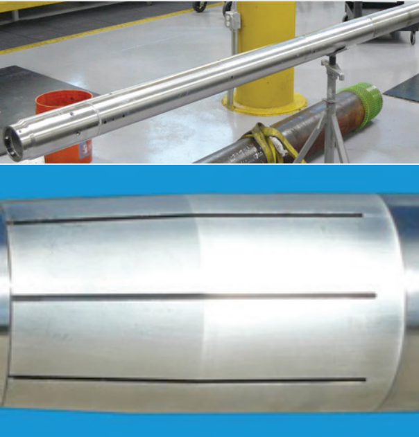
Figure 3 shows a Packer made out of alloy 945X intended for use in aggressive environment for an oil and gas well.
